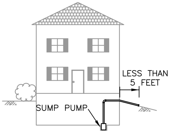
OVERLAND DISCHARGE LESS THAN 5 FEET FROM BUILDING
