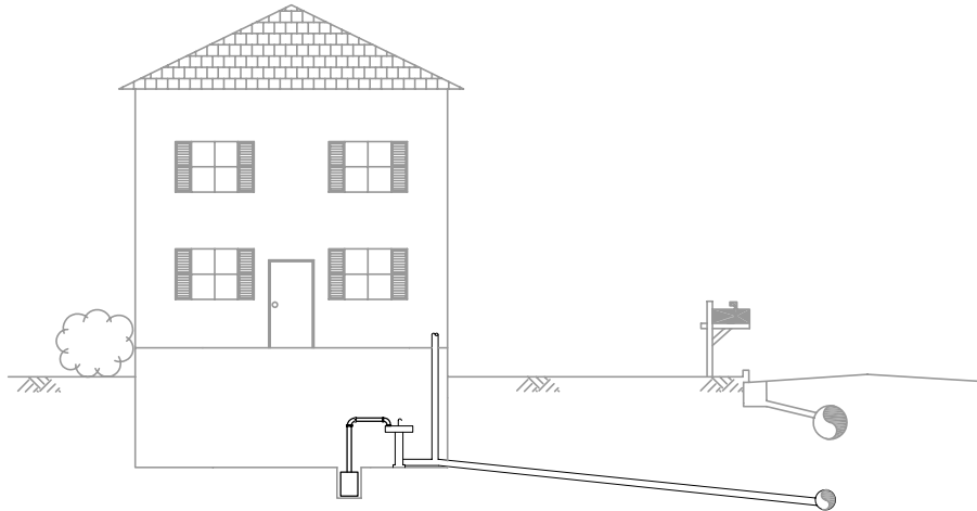
SUMP PUMP CONNECTED TO SANITARY SEWER VIA A WASH SINK
