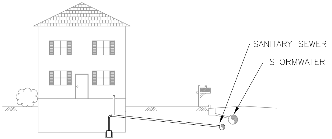
SUMP PUMP DIRECTLY CONNECTED TO SANITARY SEWER
