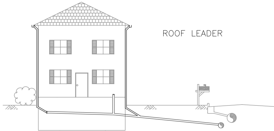
ROOF LEADERS CONNECTED TO SANITARY SEWER
