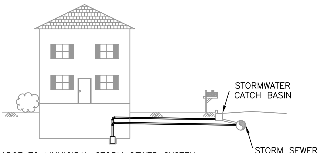
DISCHARGE TO MUNICIPAL STORM SEWER SYSTEM
