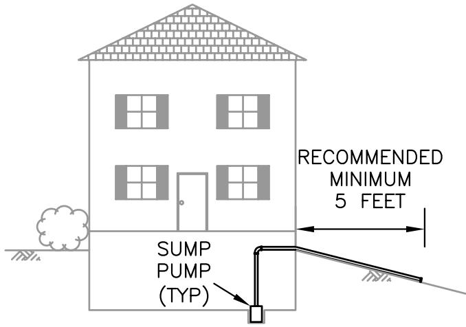
OVERLAND DISCHARGE: RECOMMENDED AT LEAST 5 FEET FROM BUILDING
